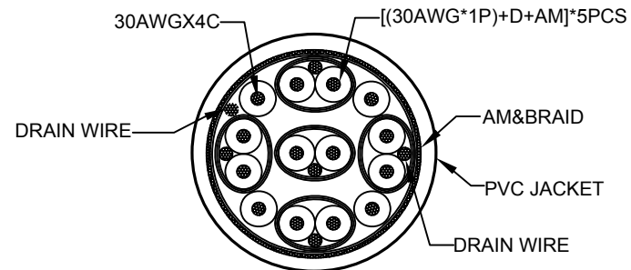
ULTRA HIGH SPEED HDMI® CABLE
